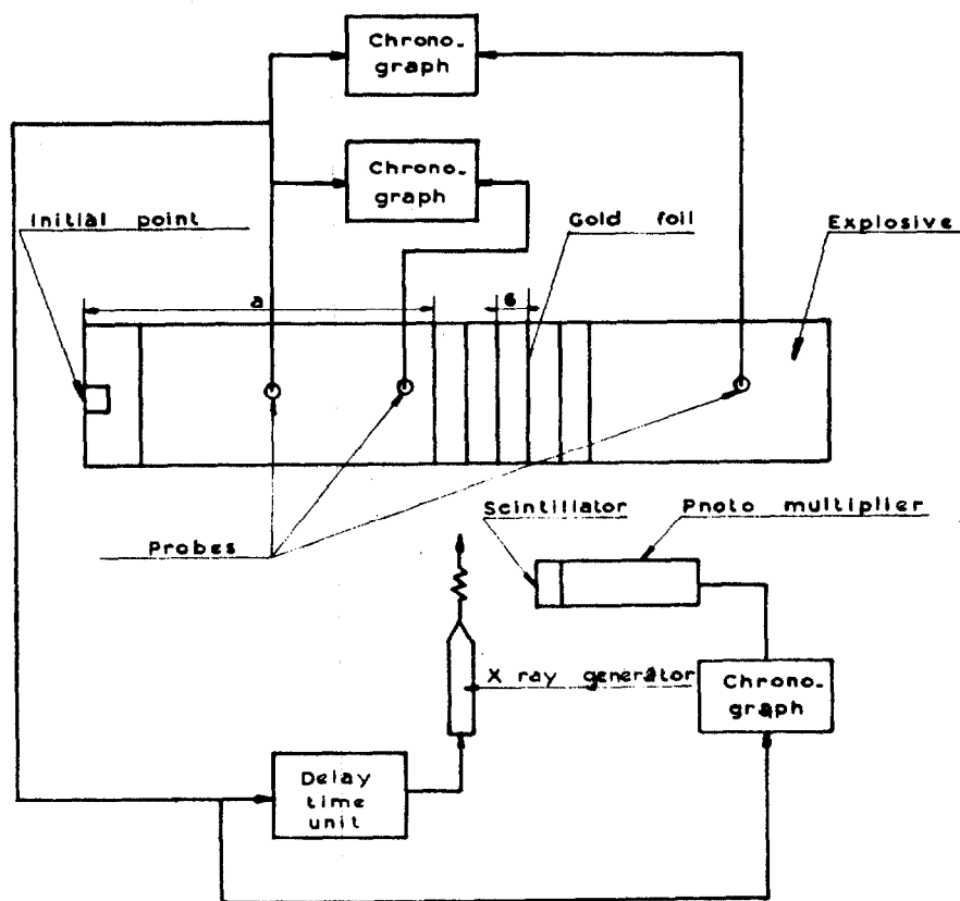
Fig 1 - Experimental arrangement
